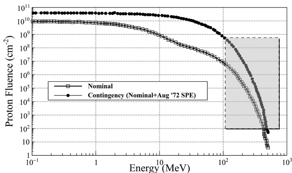
Fig. 3. Proton fluences for both the nominal and contingency test cases. The gray shaded box emphasizes the enhancement of \geq 100 MeV protons for the case where the August 1972 SPE is included in the dose projections.
