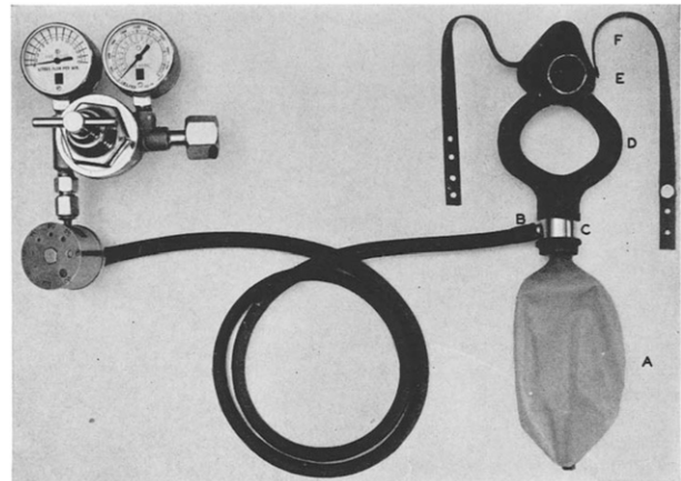
Fig. 1. Injector attached to oxygen regulator and nasal mask.
